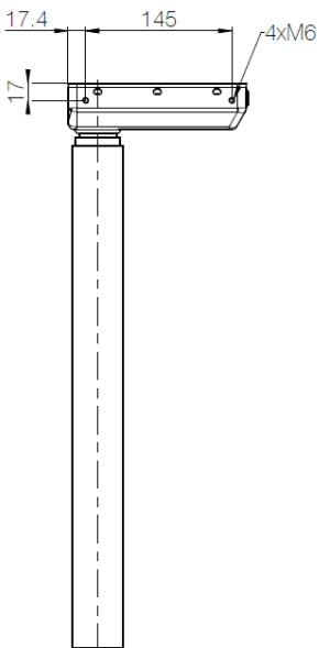
DL6 dimensions (mm)
