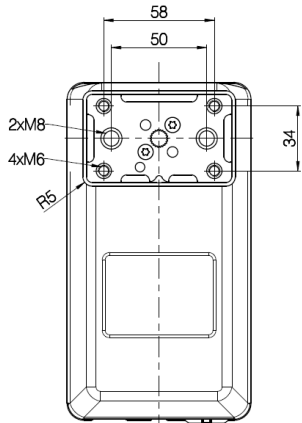
Bottom plate
